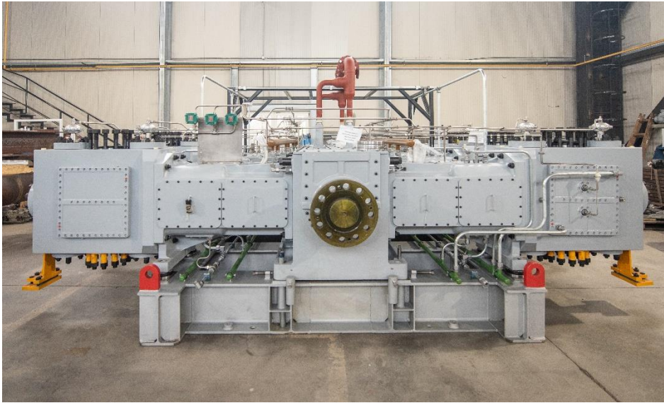
Image 3: Built with adaptability in mind, the HS-C/HS-E New Build Compressor Packages can accommodate a wide range of footprints and cylinder configurations.
