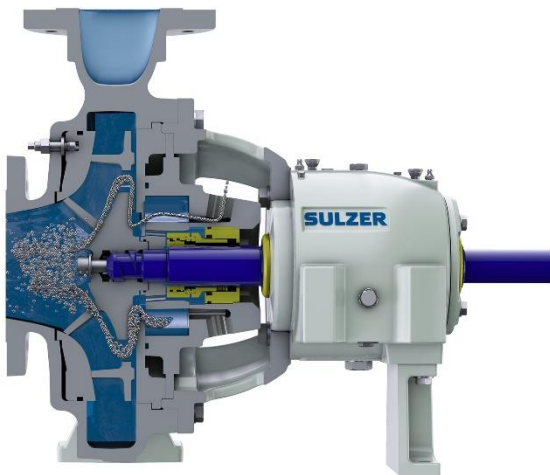
Image 2: AHLSTAR A-LM pump
