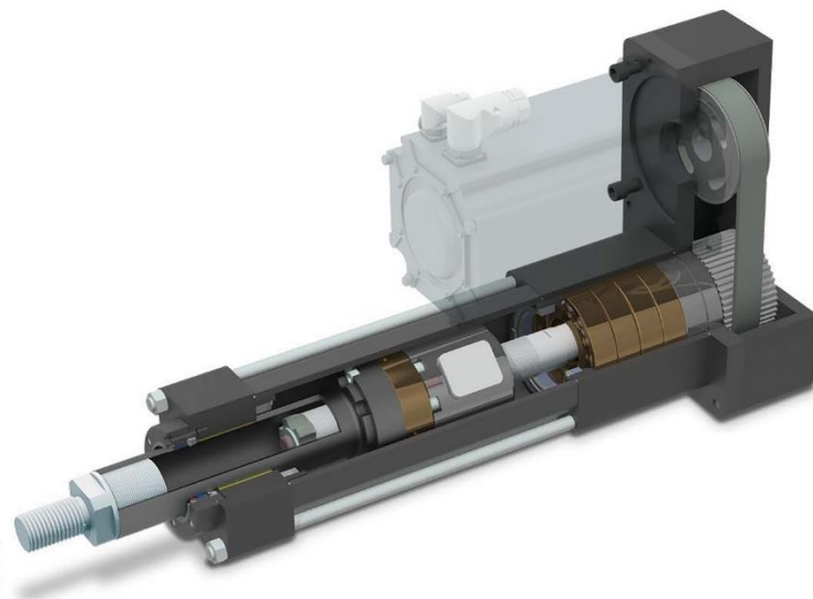
Image 2: RSX actuators are available with Ball and Planetary roller screw driven designs to fit application requirements, ensuring consistency over an extended service life.
