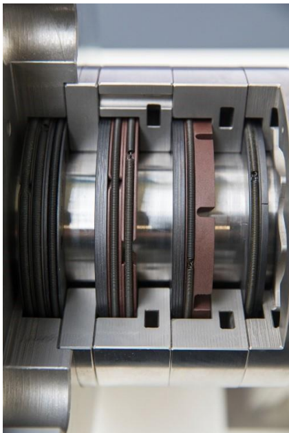
Image 2: Material, design and arrangement of rings is important to achieve highest reliability.
